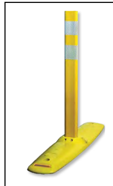
Typical surface mounted turnpike curb with delineators in white
