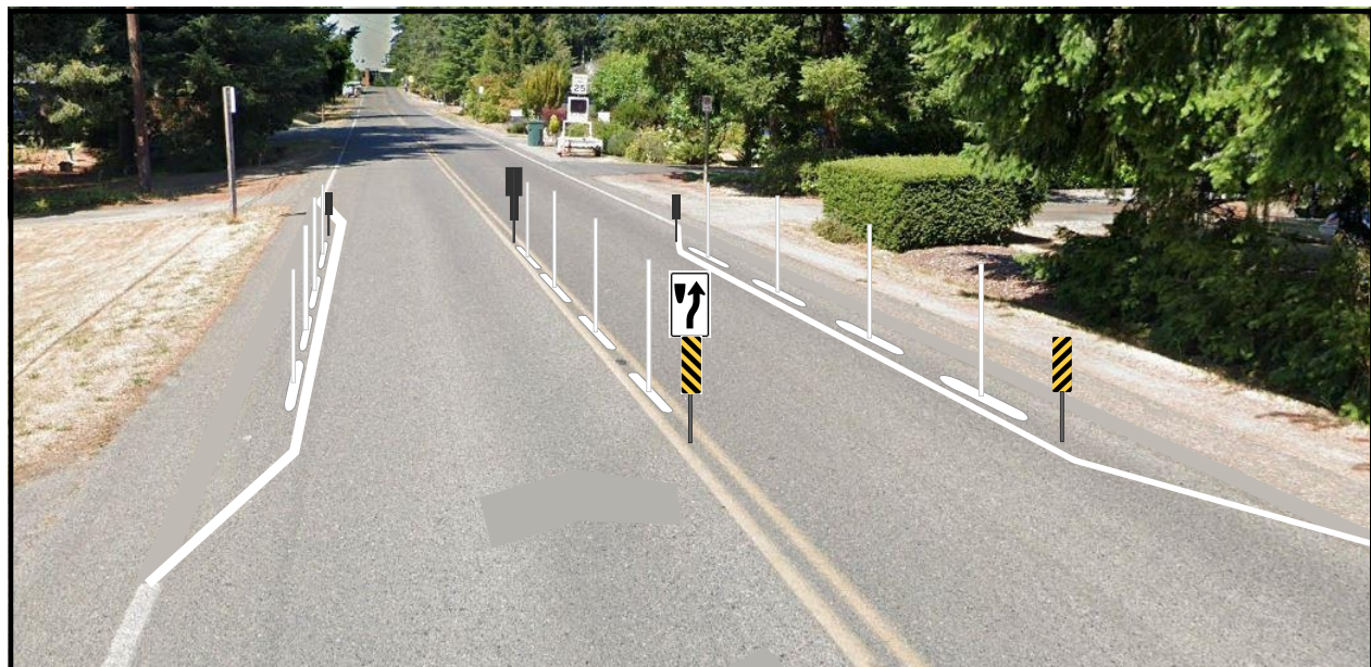
SLOW POINT TYPICAL LAYOUT ON GROW AVENUE (LOOKING NORTH)
