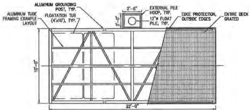
BOARDING FLOAT PLAN EXAMPLE
