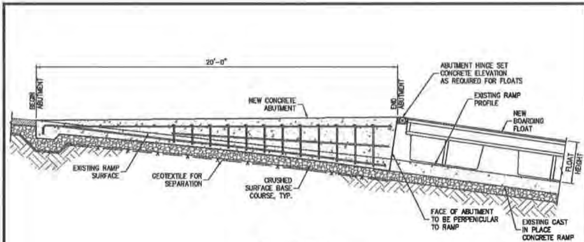
PROPOSED ABUTMENT PROFILE
