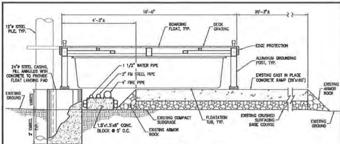
SECTION A-A BOARDING FLOAT & RAMP
