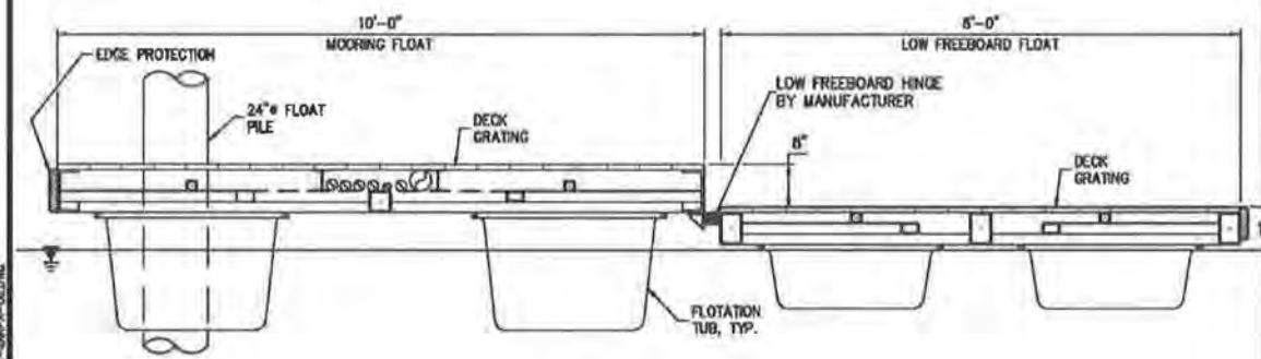
SECTION B-B MOORING & LOW FREEBOARD FLOATS
