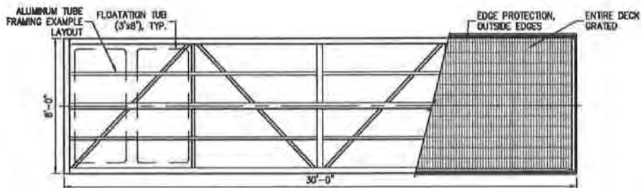
LOW FREEBOARD FLOAT PLAN EXAMPLE
