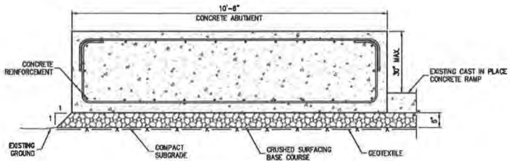
PROPOSED ABUTMENT SECTION
